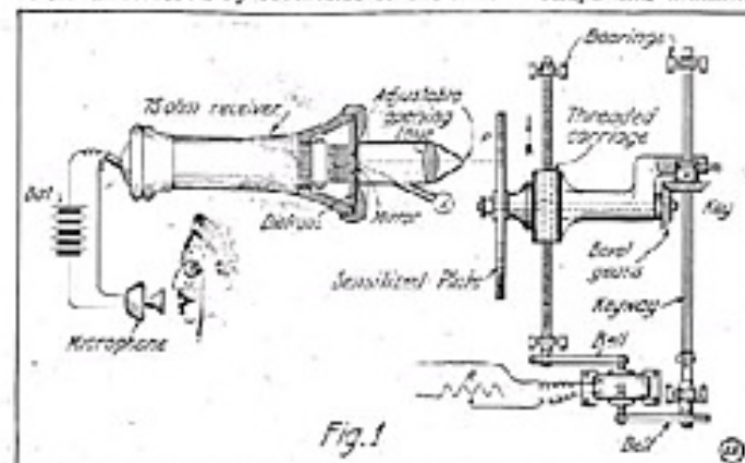
Scheme for recording the voice photographically.
