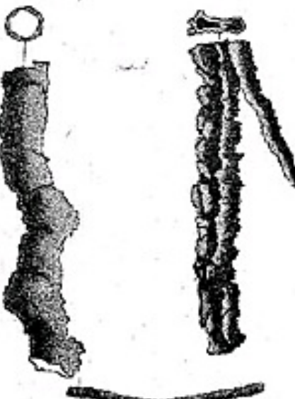
Showing the Very Peculiar and Striking Ferris Produced in Sand When Lightning Strikes It. Sometimes Called Lightning Tubes.
