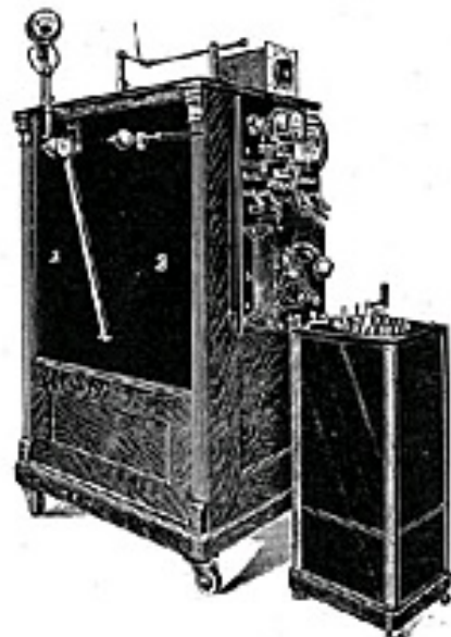
Fig. 1A. Appearance of Modern 100,000 Volt X-Ray Generator Delivering Direct Current.
