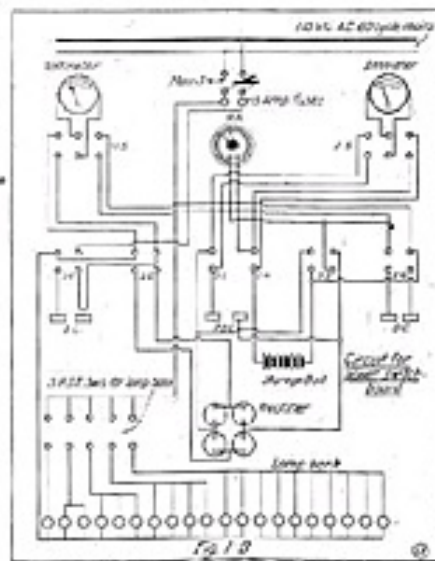
Circuits for 110 Volt A. C. Switch-board.
