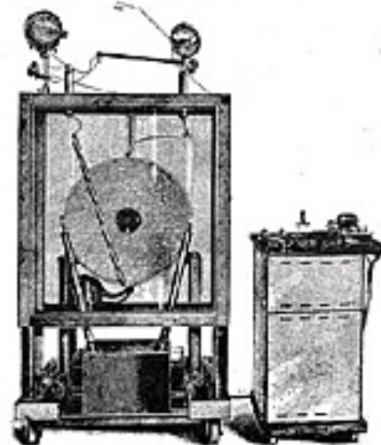
Fig. 5. Heavy Current Interrupterless X-Ray Generator. Micanite Disc is Seen Enclosed in Glass Cabinet, 100,000 Volt Transformer at Base.
