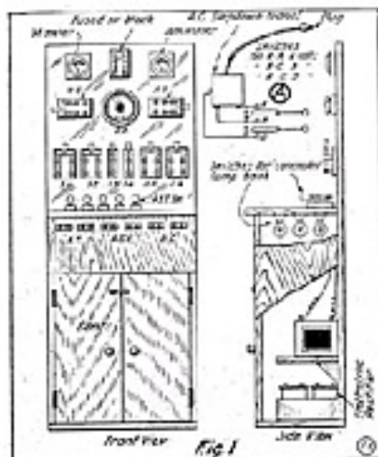
Front and Side View of 110 Volt Switch-board.
