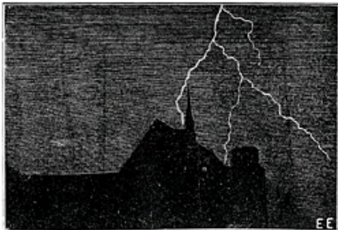
Showing a Single Stroke of Lightning From Cloud to Earth. A Return Stroke From Earth to Cloud Often Occurs. Hence the Futility of Staying in a Cellar.
