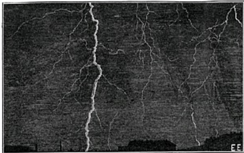
Spectacular Illustration of Lightning. Note the Several Divided Branches of the Discharges. Such Flashes May Involve Millions of Volts and Thousands of Horsepower.
